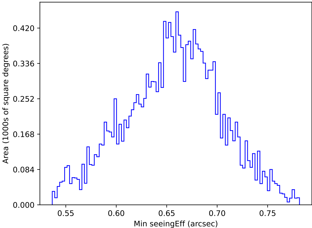
too_elab_r16_d2_ugrizy_v3.4_10yrs WFD g band: Min seeingEff
