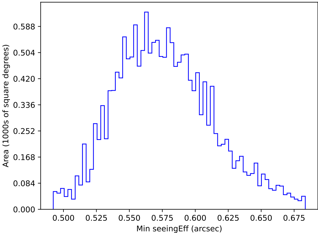
too_elab_r16_d2_ugrizy_v3.4_10yrs WFD all bands: Min seeingEff
