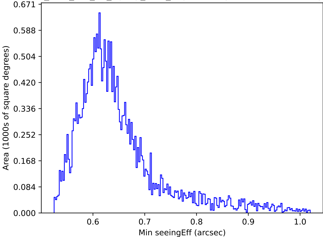
too_elab_r16_d2_ugrizy_v3.4_10yrs All sky z band: Min seeingEff
