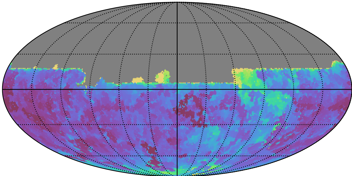
too_elab_r16_d2_ugrizy_v3.4_10yrs All sky u band: Min seeingEff
