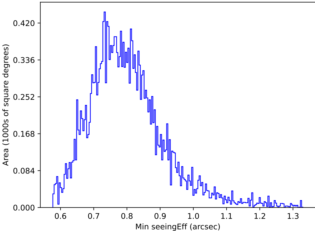
too_elab_r16_d2_ugrizy_v3.4_10yrs All sky u band: Min seeingEff
