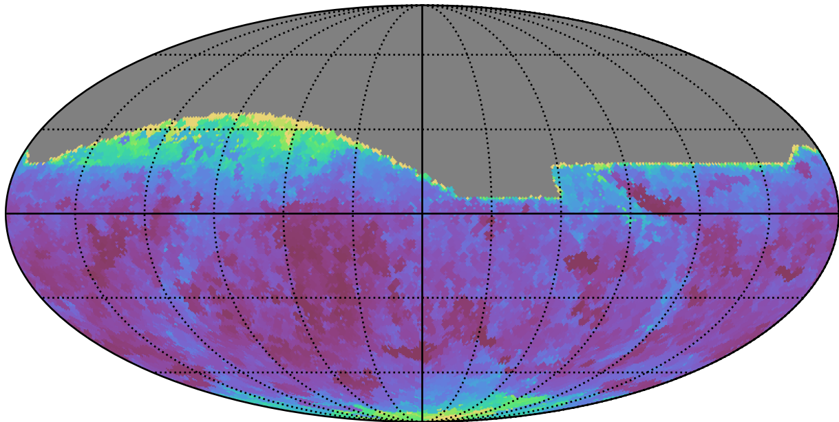
too_elab_r16_d2_ugrizy_v3.4_10yrs All sky i band: Min seeingEff
