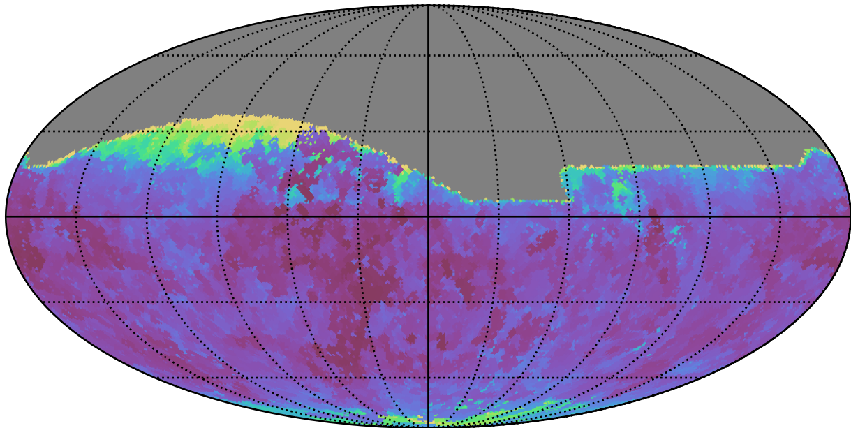
too_elab_r16_d2_ugrizy_v3.4_10yrs All sky g band: Min seeingEff
