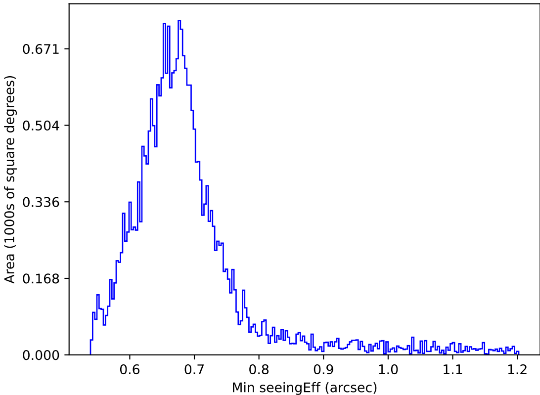
too_elab_r16_d2_ugrizy_v3.4_10yrs All sky g band: Min seeingEff
