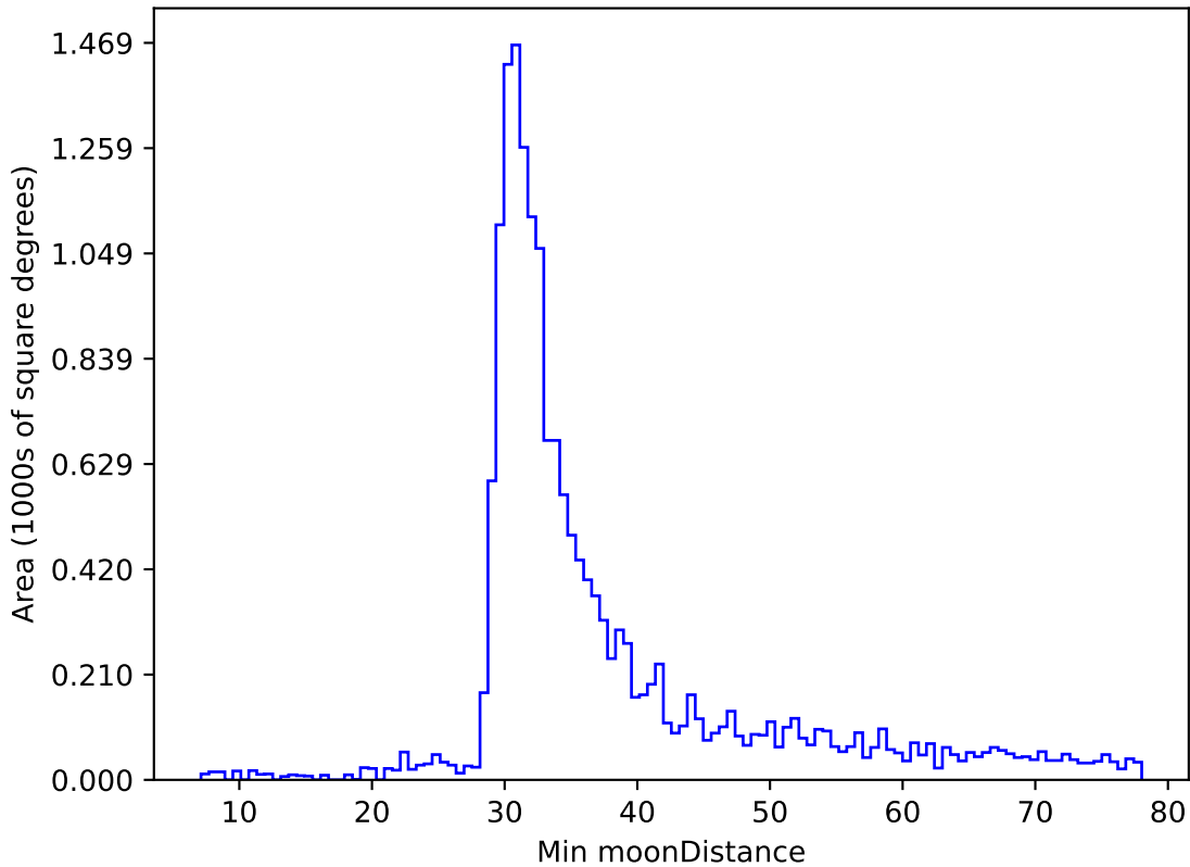
too_elab_r16_d2_ugrizy_v3.4_10yrs WFD r band: Min moonDistance
