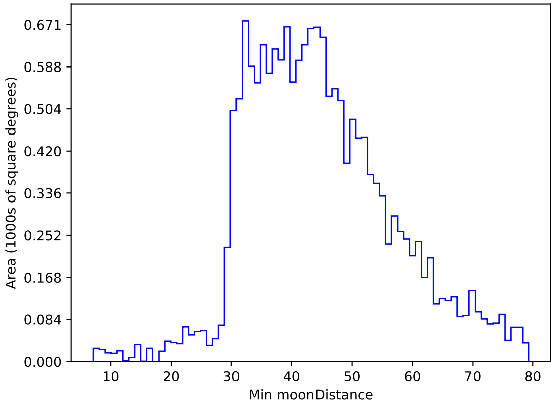
too_elab_r16_d2_ugrizy_v3.4_10yrs WFD g band: Min moonDistance
