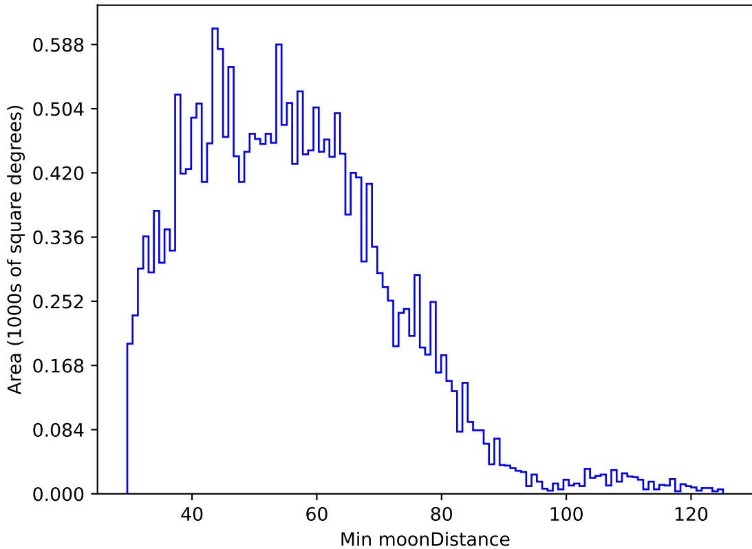
too_elab_r16_d2_ugrizy_v3.4_10yrs All sky u band: Min moonDistance
