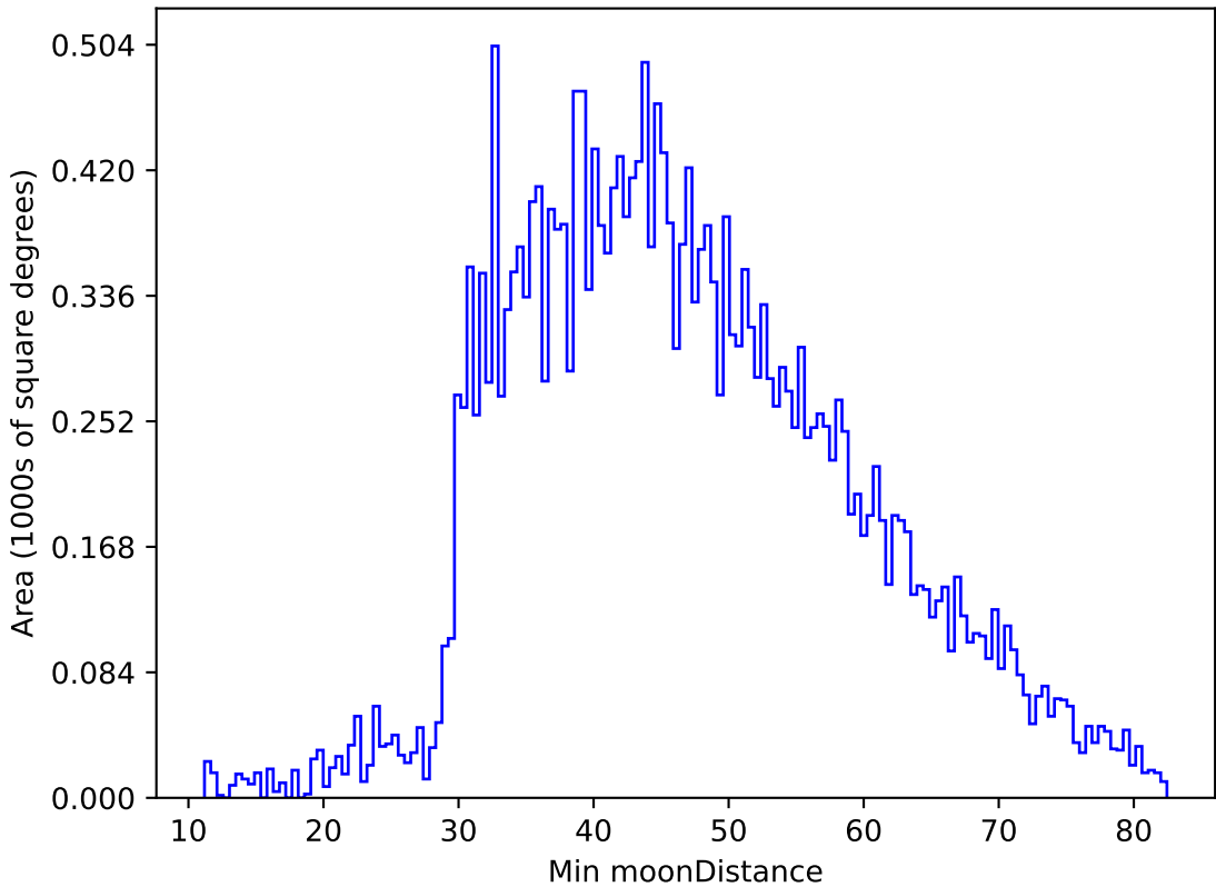
too_elab_r16_d2_ugrizy_v3.4_10yrs All sky g band: Min moonDistance
