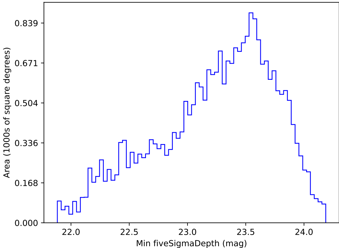
too_elab_r16_d2_ugrizy_v3.4_10yrs Yr 1 r band: Min fiveSigmaDepth
