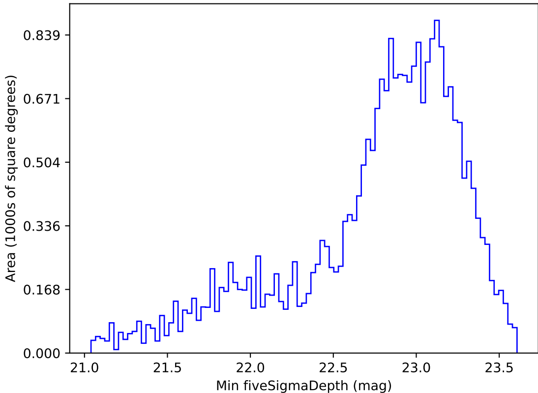
too_elab_r16_d2_ugrizy_v3.4_10yrs Yr 1 i band: Min fiveSigmaDepth
