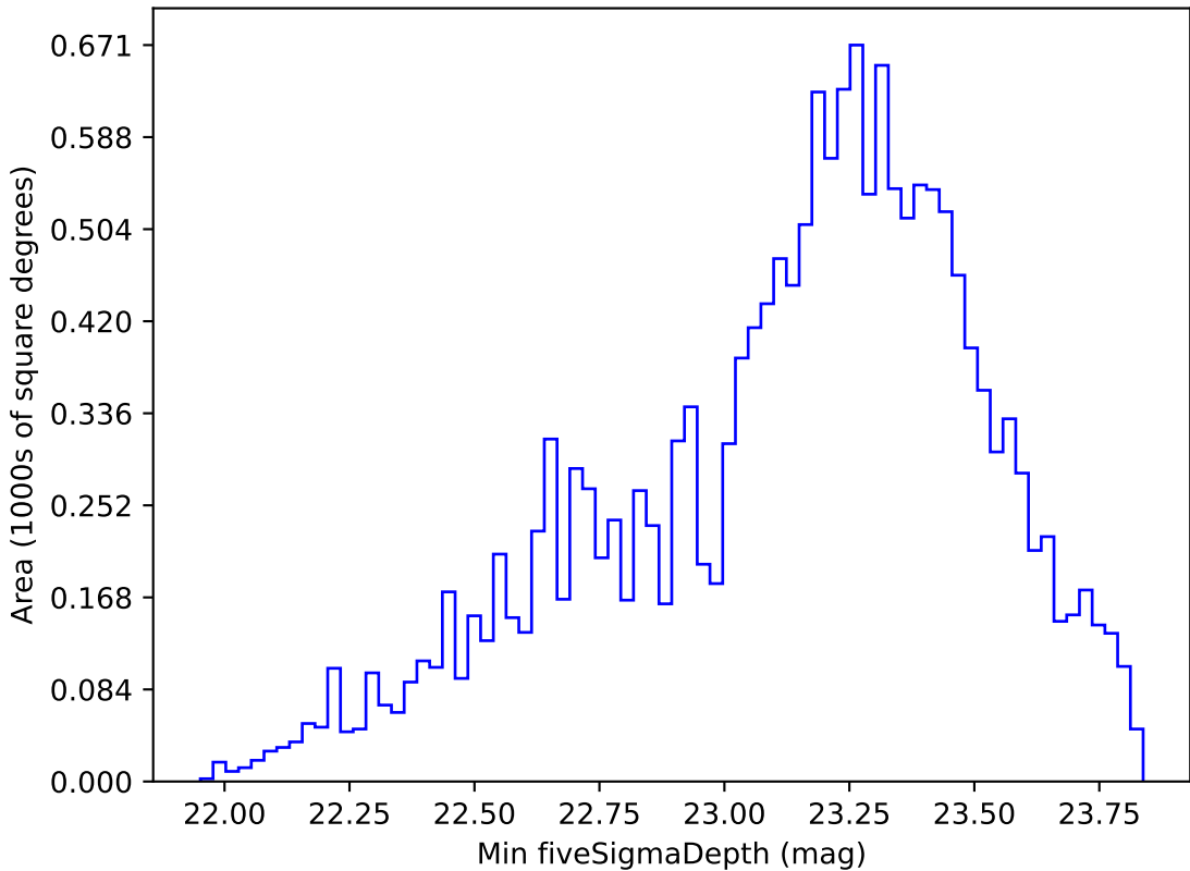
too_elab_r16_d2_ugrizy_v3.4_10yrs WFD g band: Min fiveSigmaDepth
