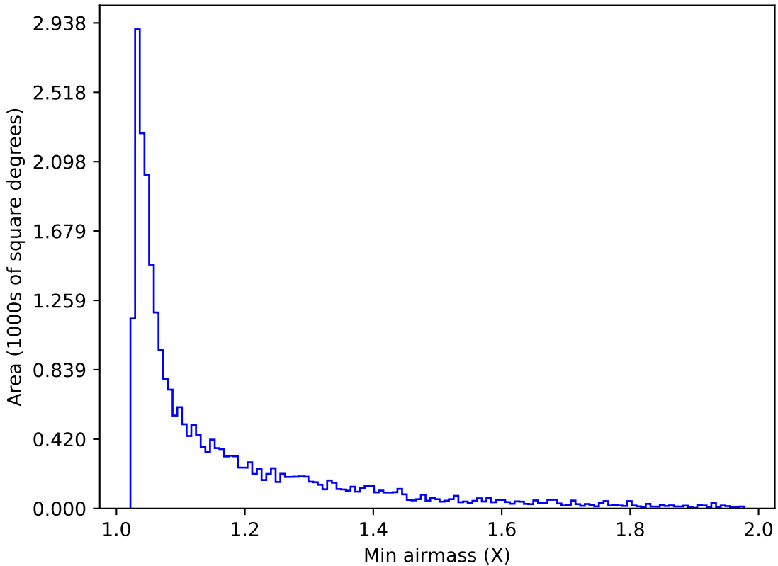
too_elab_r16_d2_ugrizy_v3.4_10yrs Yr 1 z band: Min airmass
