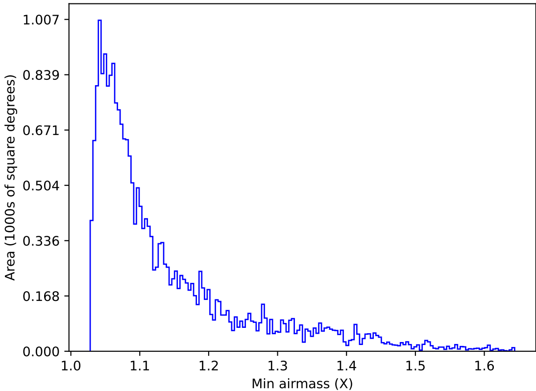
too_elab_r16_d2_ugrizy_v3.4_10yrs Yr 1 u band: Min airmass
