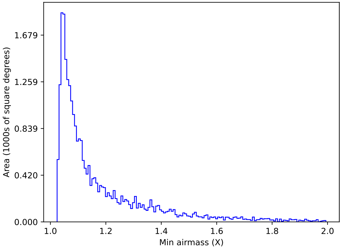
too_elab_r16_d2_ugrizy_v3.4_10yrs Yr 1 g band: Min airmass
