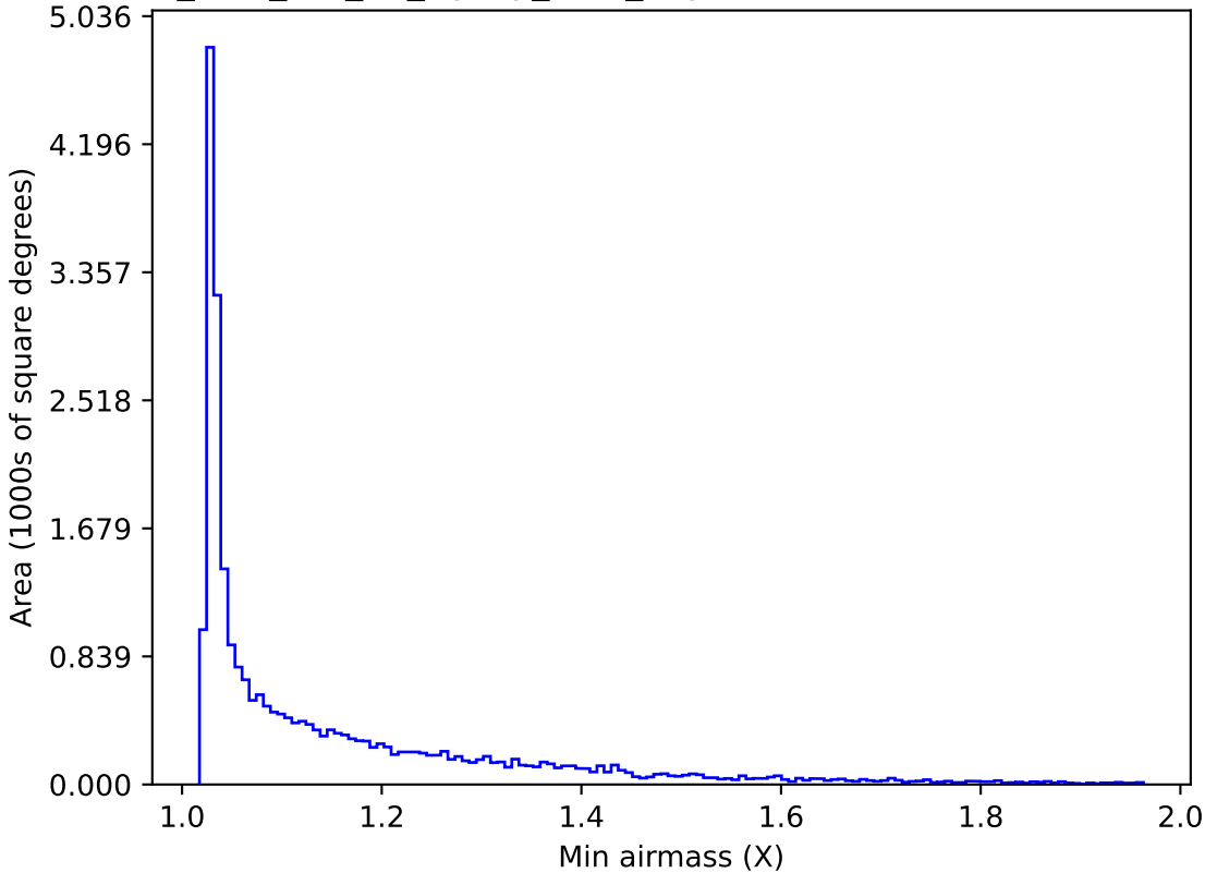
too_elab_r16_d2_ugrizy_v3.4_10yrs Yr 1 all bands: Min airmass
