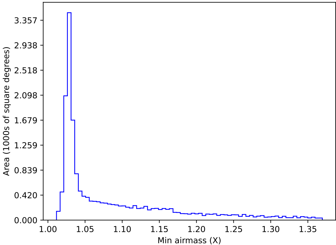
too_elab_r16_d2_ugrizy_v3.4_10yrs WFD z band: Min airmass
