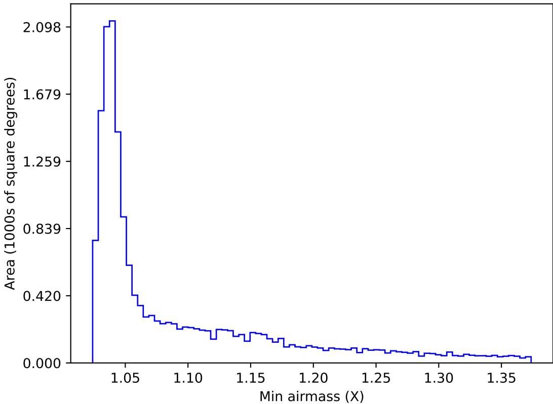
too_elab_r16_d2_ugrizy_v3.4_10yrs WFD u band: Min airmass
