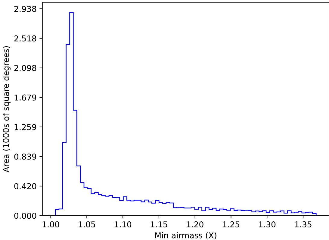
too_elab_r16_d2_ugrizy_v3.4_10yrs WFD r band: Min airmass
