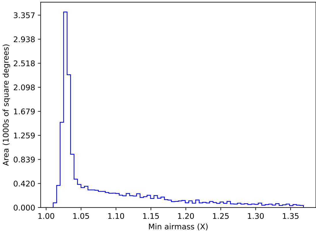
too_elab_r16_d2_ugrizy_v3.4_10yrs WFD i band: Min airmass
