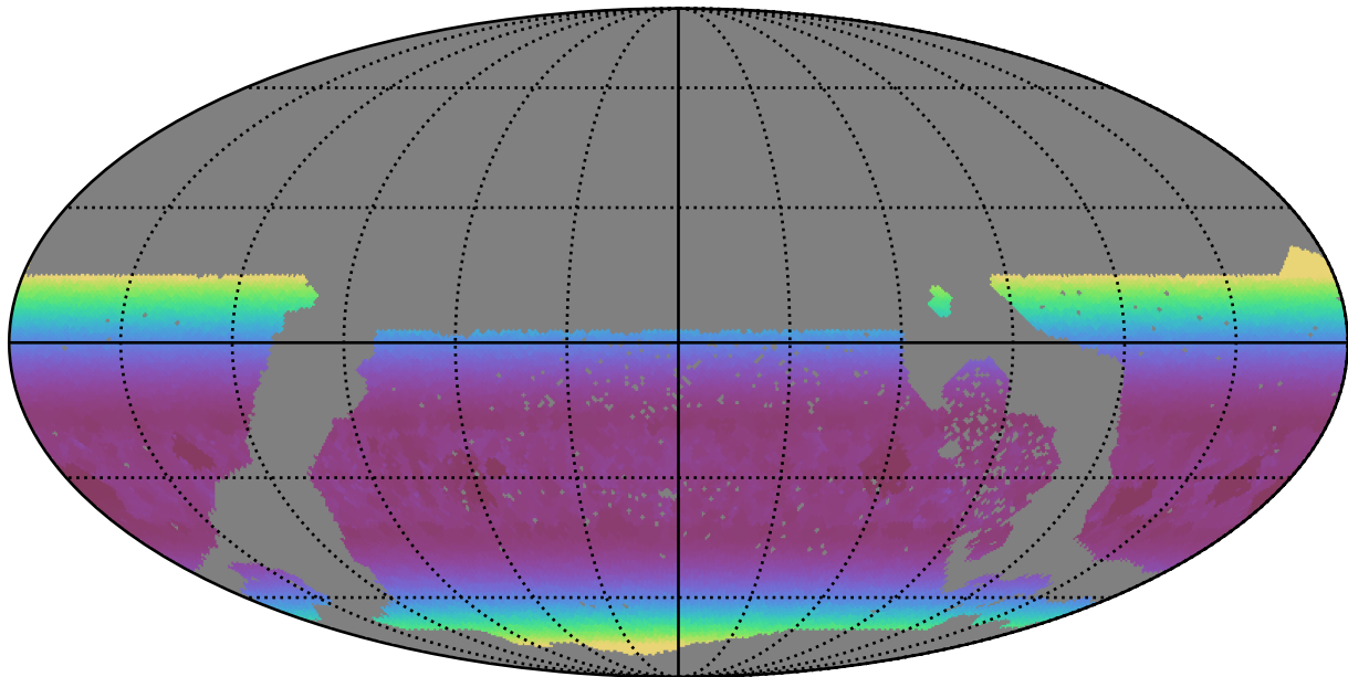
too_elab_r16_d2_ugrizy_v3.4_10yrs WFD g band: Min airmass
