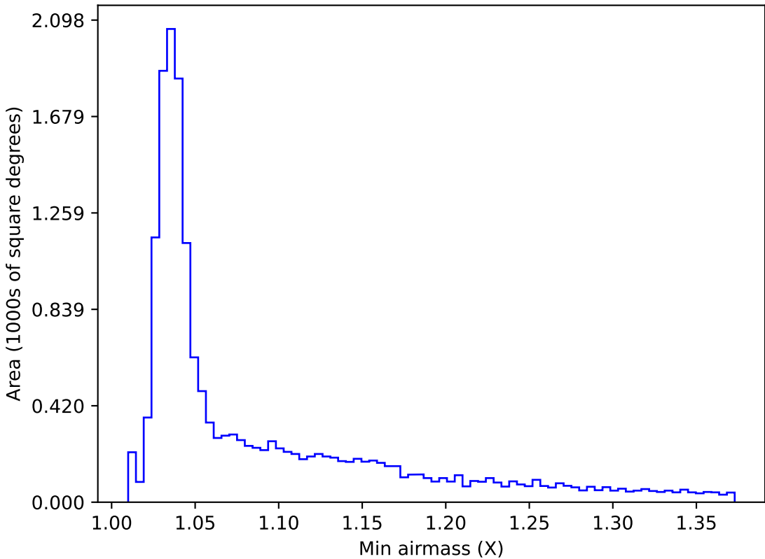
too_elab_r16_d2_ugrizy_v3.4_10yrs WFD g band: Min airmass
