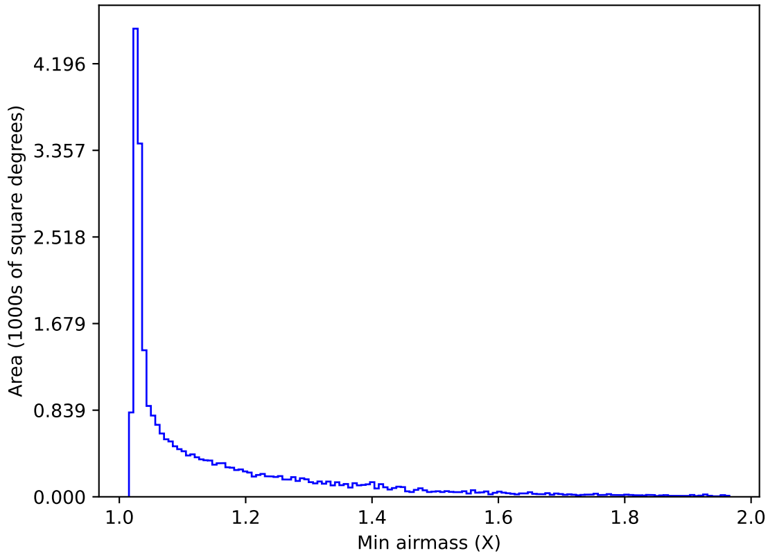
too_elab_r16_d2_ugrizy_v3.4_10yrs All sky z band: Min airmass
