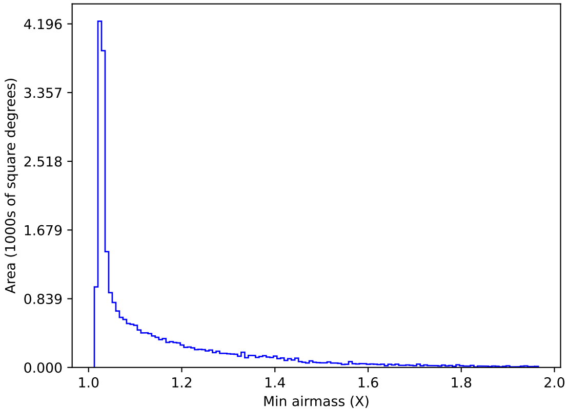
too_elab_r16_d2_ugrizy_v3.4_10yrs All sky r band: Min airmass
