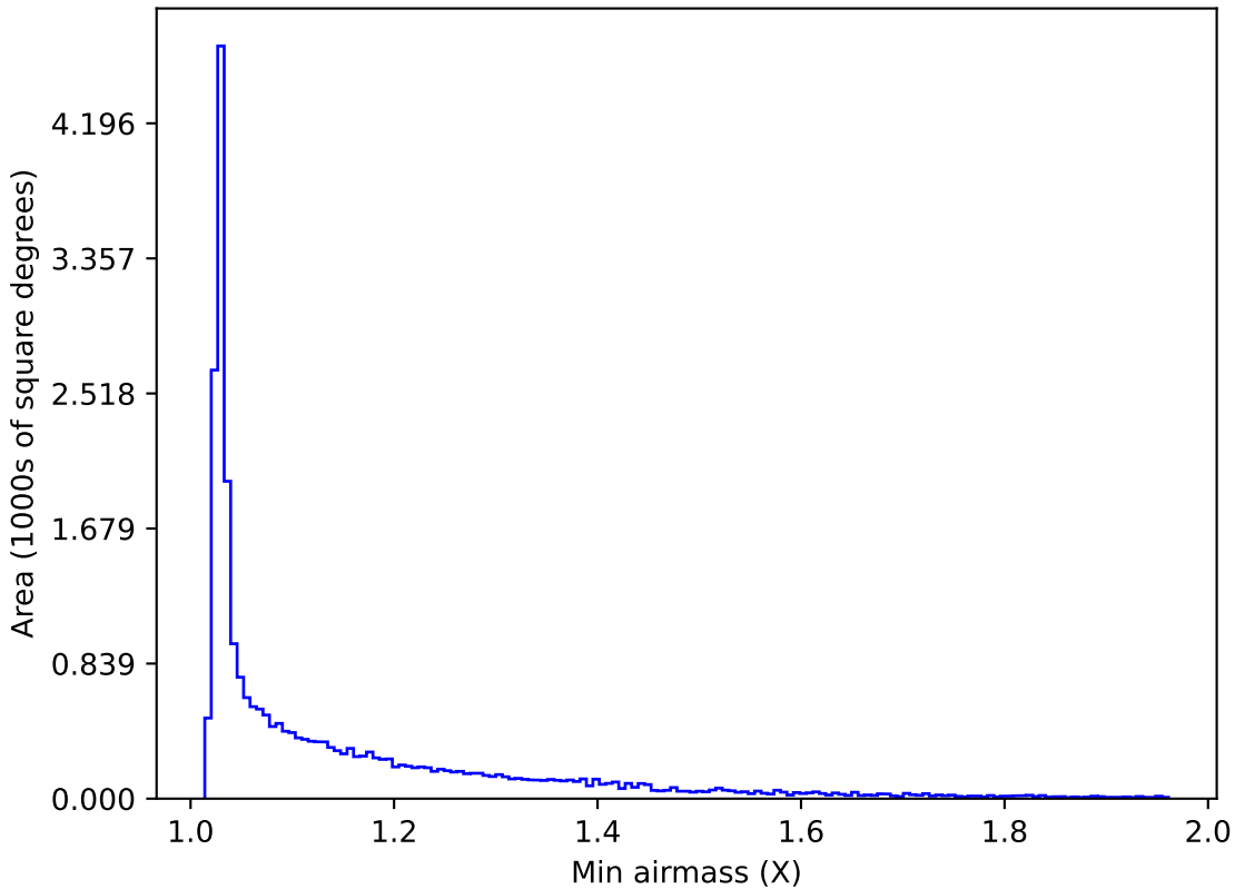
too_elab_r16_d2_ugrizy_v3.4_10yrs All sky i band: Min airmass
