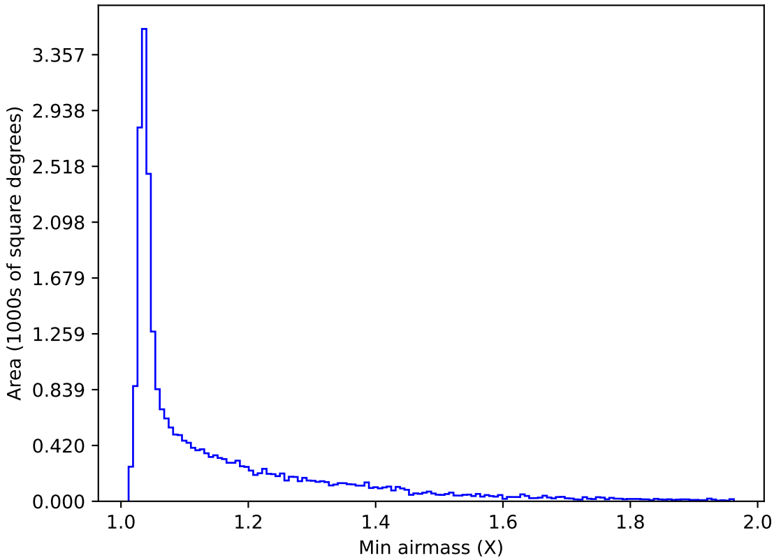
too_elab_r16_d2_ugrizy_v3.4_10yrs All sky g band: Min airmass
