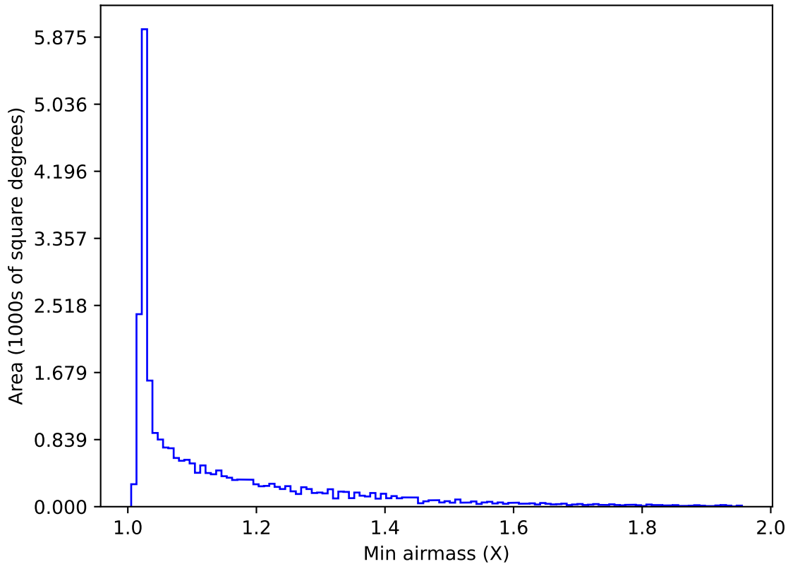
too_elab_r16_d2_ugrizy_v3.4_10yrs All sky all bands: Min airmass
