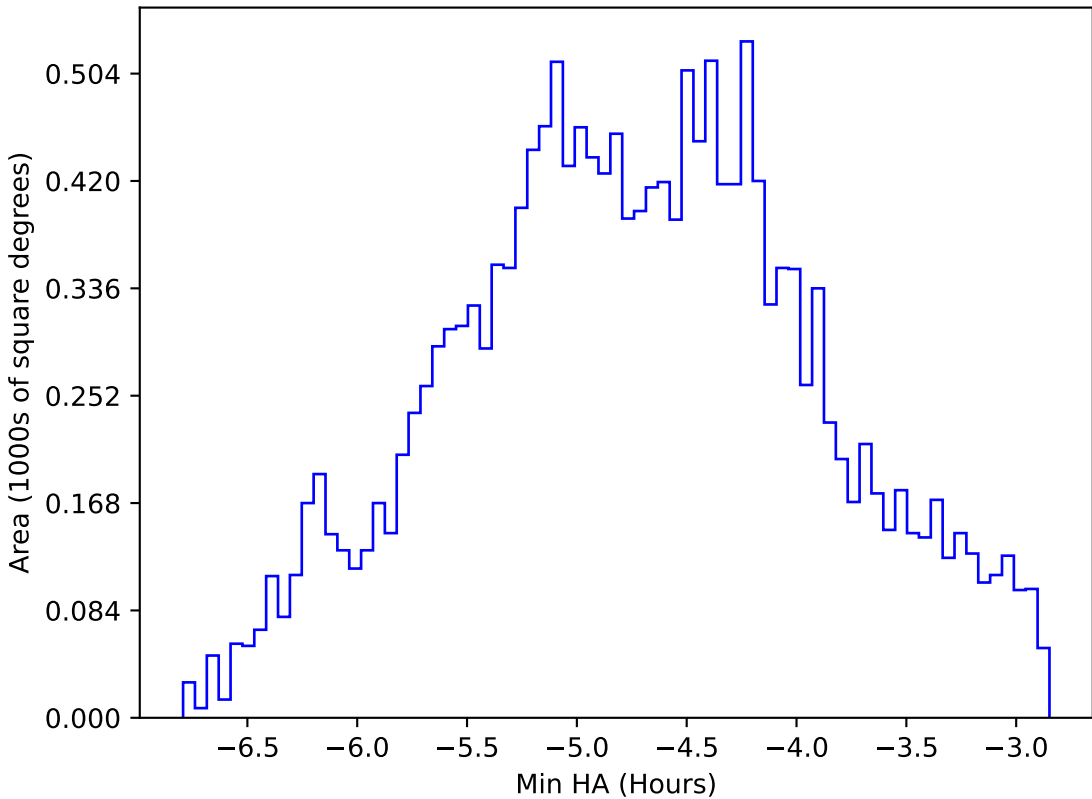
too_elab_r16_d2_ugrizy_v3.4_10yrs WFD all bands: Min HA
