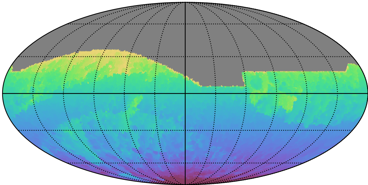
too_elab_r16_d2_ugrizy_v3.4_10yrs All sky all bands: Min HA
