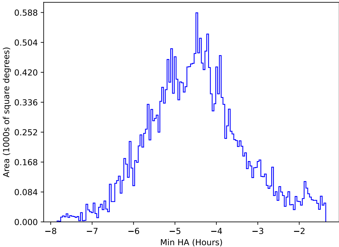
too_elab_r16_d2_ugrizy_v3.4_10yrs All sky all bands: Min HA
