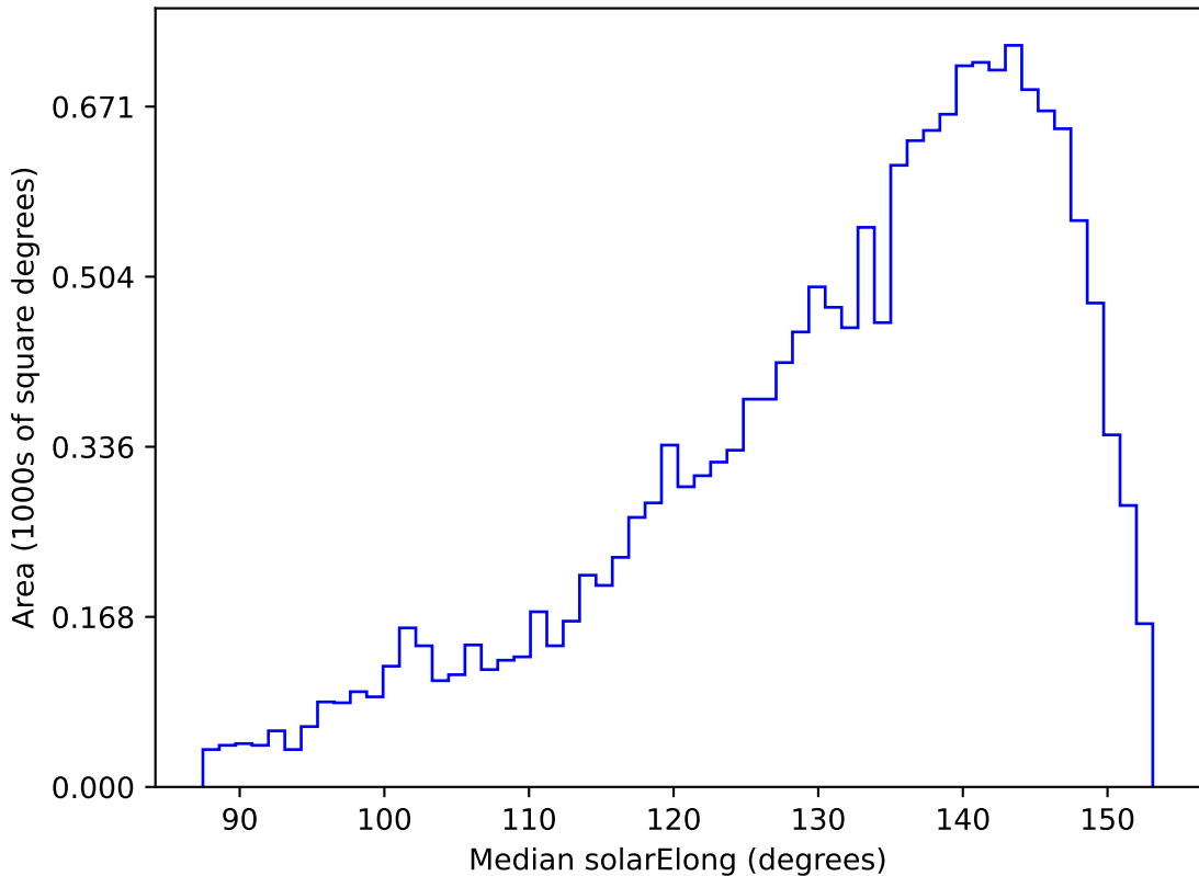
too_elab_r16_d2_ugrizy_v3.4_10yrs WFD u band: Median solarElong
