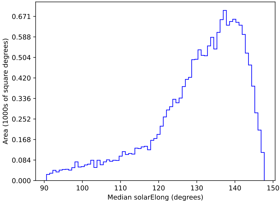
too_elab_r16_d2_ugrizy_v3.4_10yrs WFD r band: Median solarElong
