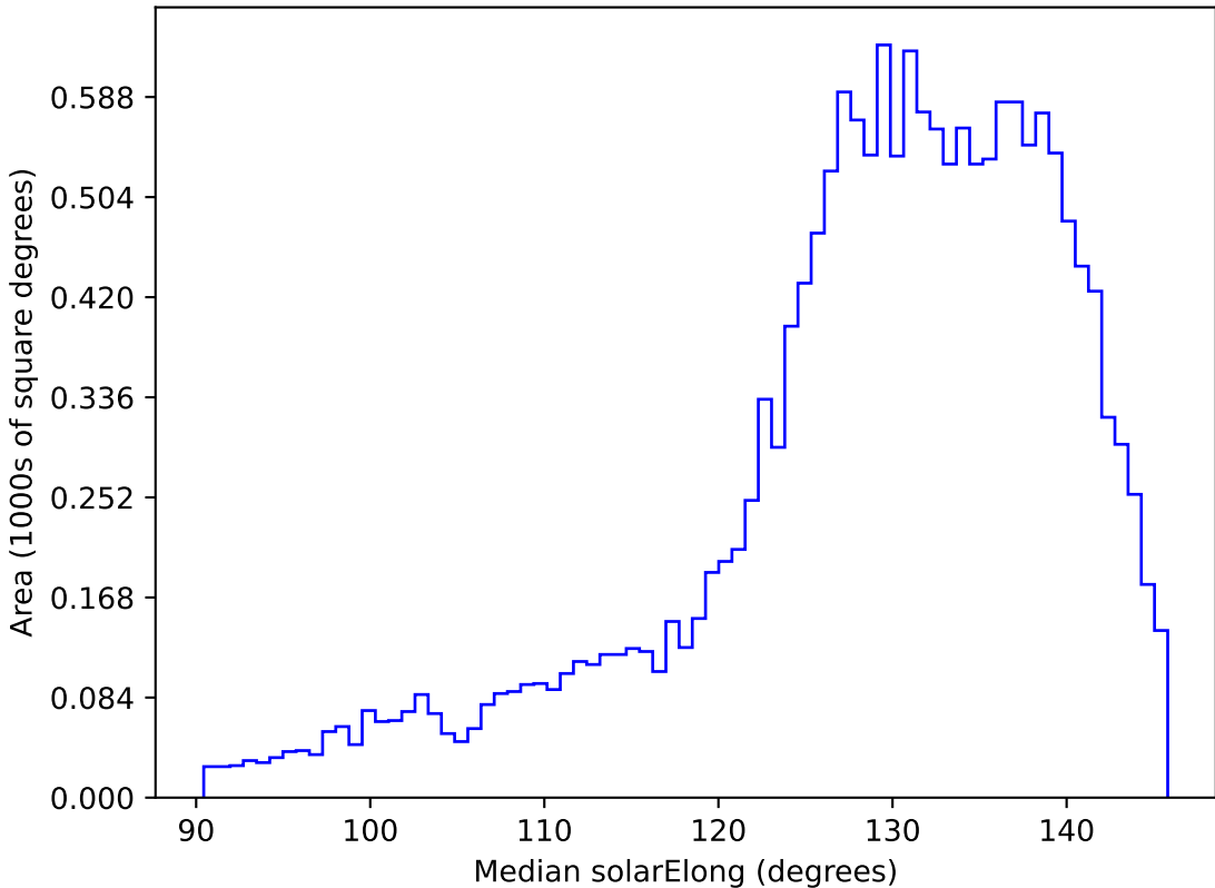
too_elab_r16_d2_ugrizy_v3.4_10yrs WFD i band: Median solarElong
