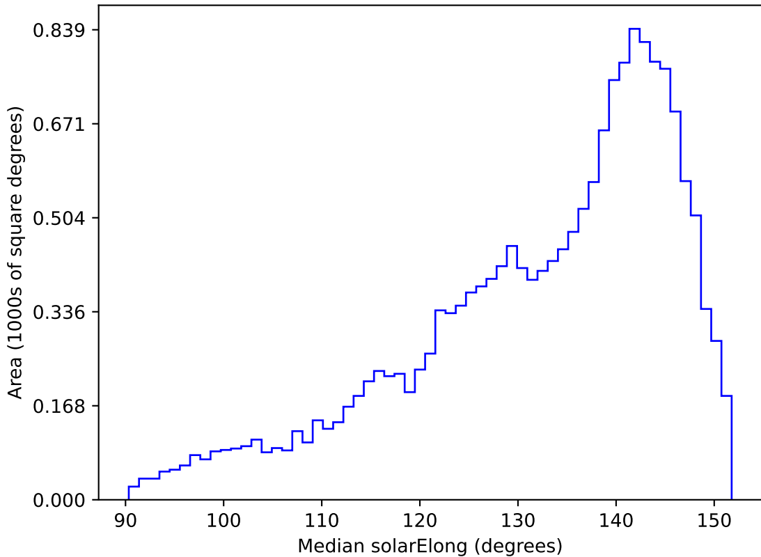
too_elab_r16_d2_ugrizy_v3.4_10yrs WFD g band: Median solarElong
