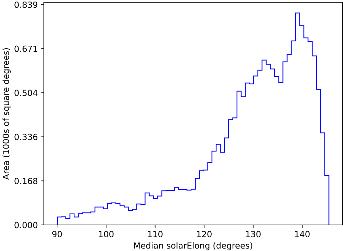
too_elab_r16_d2_ugrizy_v3.4_10yrs WFD all bands: Median solarElong
