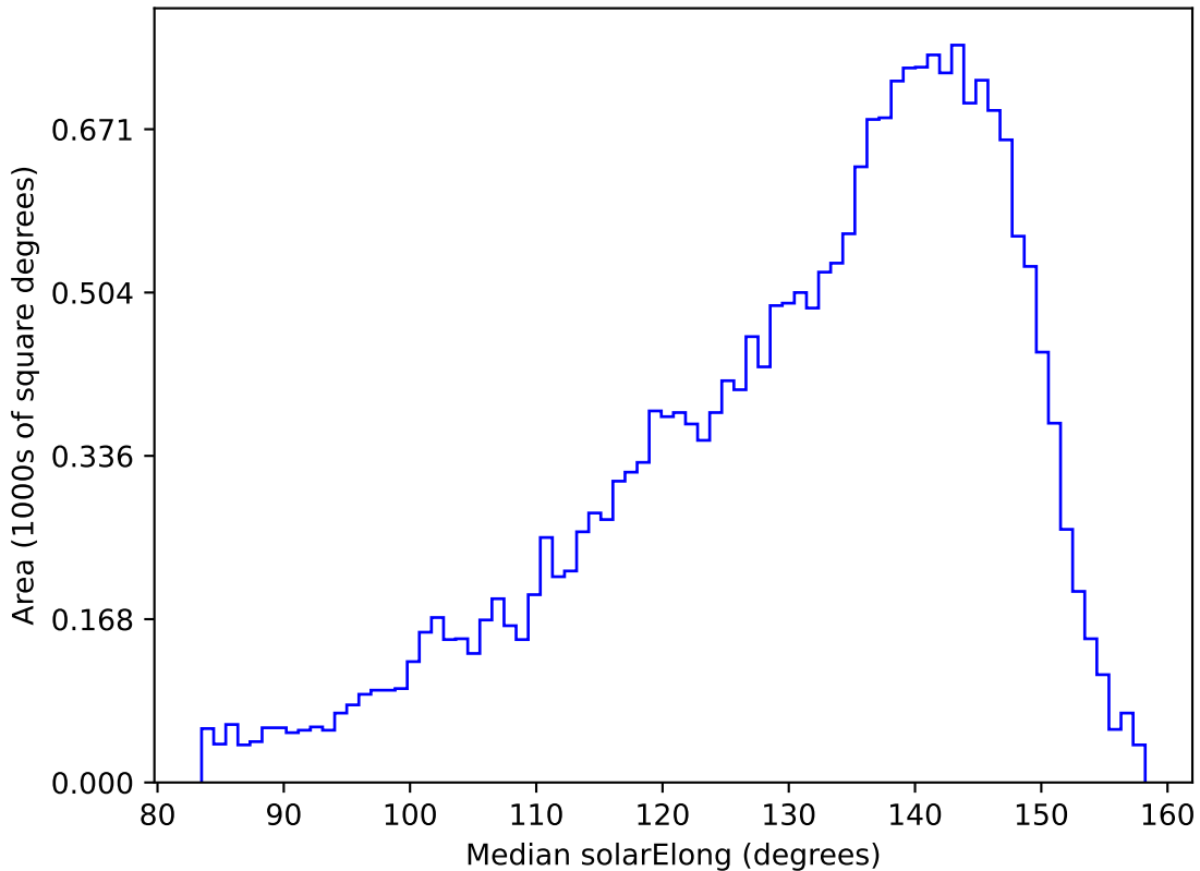
too_elab_r16_d2_ugrizy_v3.4_10yrs All sky u band: Median solarElong
