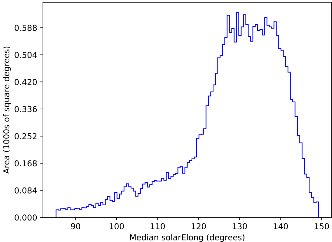
too_elab_r16_d2_ugrizy_v3.4_10yrs All sky i band: Median solarElong
