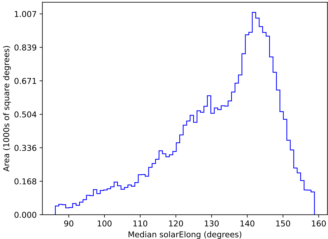
too_elab_r16_d2_ugrizy_v3.4_10yrs All sky g band: Median solarElong
