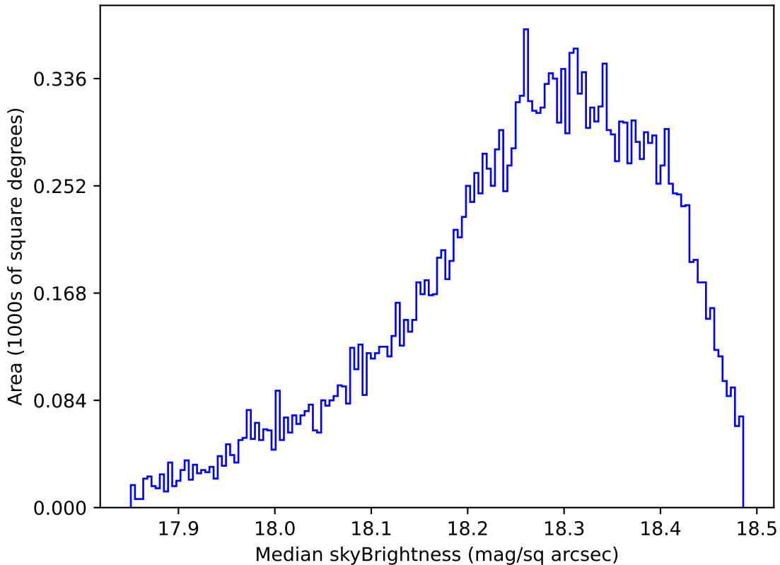
too_elab_r16_d2_ugrizy_v3.4_10yrs Yr 1 y band: Median skyBrightness
