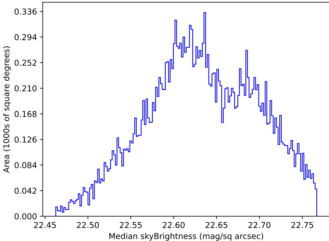
too_elab_r16_d2_ugrizy_v3.4_10yrs Yr 1 u band: Median skyBrightness
