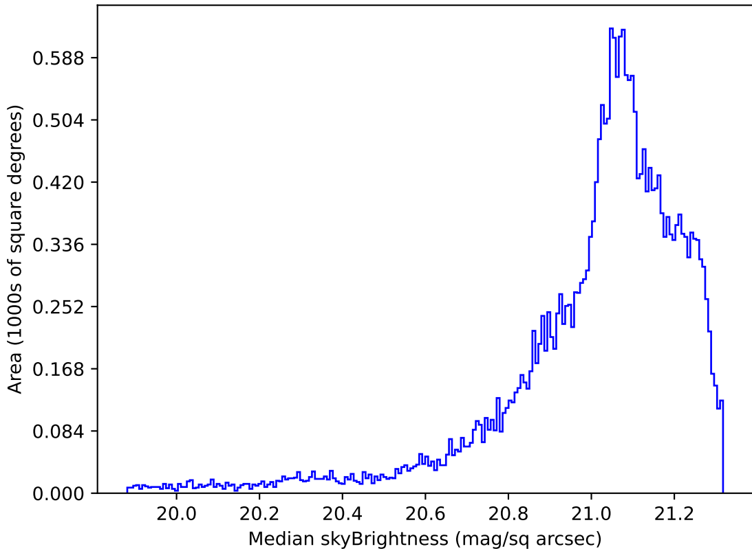
too_elab_r16_d2_ugrizy_v3.4_10yrs Yr 1 r band: Median skyBrightness
