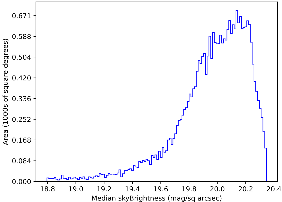
too_elab_r16_d2_ugrizy_v3.4_10yrs Yr 1 i band: Median skyBrightness
