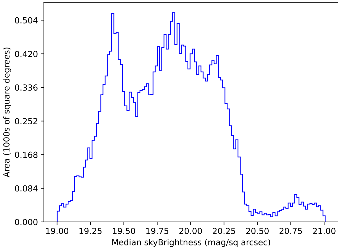
too_elab_r16_d2_ugrizy_v3.4_10yrs Yr 1 all bands: Median skyBrightness
