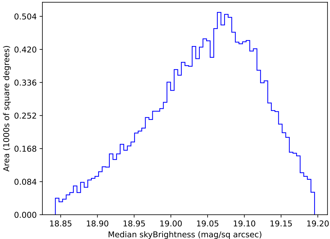
too_elab_r16_d2_ugrizy_v3.4_10yrs WFD z band: Median skyBrightness
