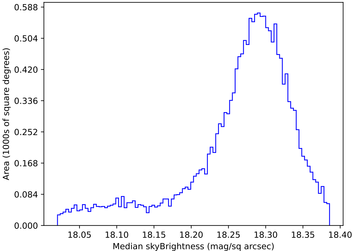
too_elab_r16_d2_ugrizy_v3.4_10yrs WFD y band: Median skyBrightness
