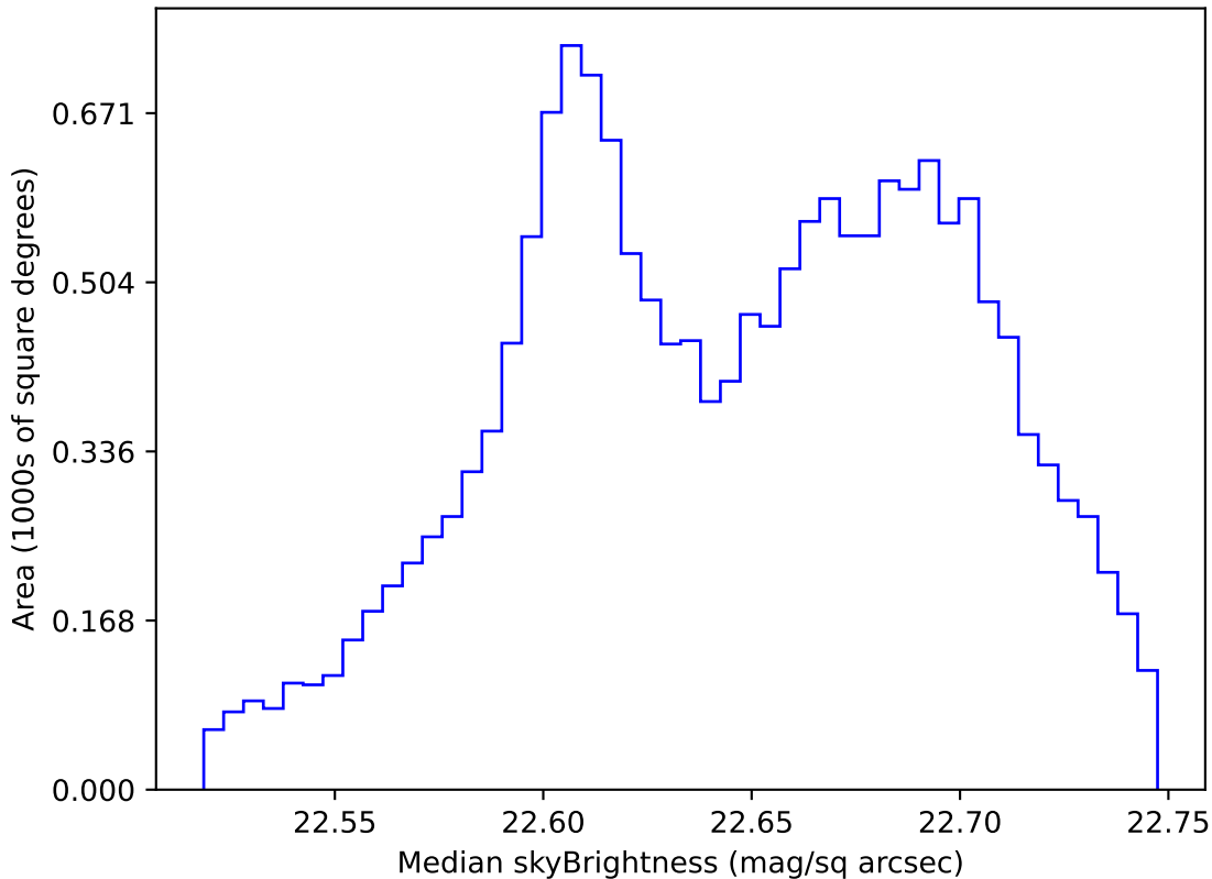
too_elab_r16_d2_ugrizy_v3.4_10yrs WFD u band: Median skyBrightness
