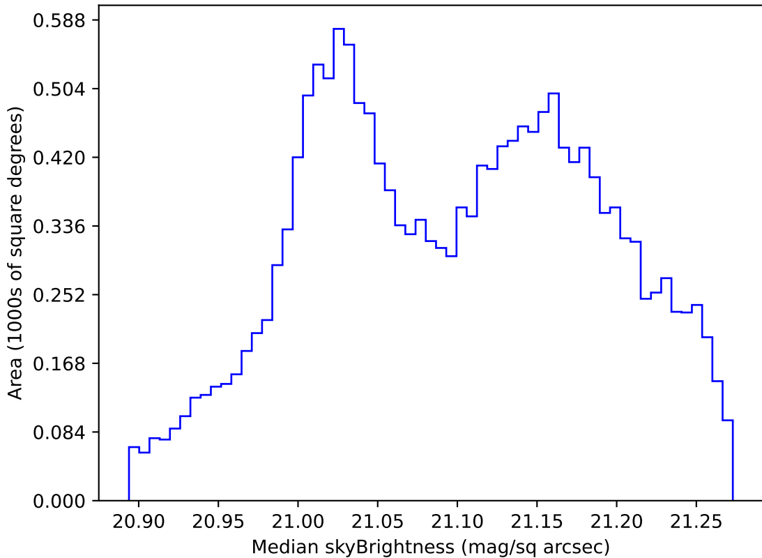
too_elab_r16_d2_ugrizy_v3.4_10yrs WFD r band: Median skyBrightness
